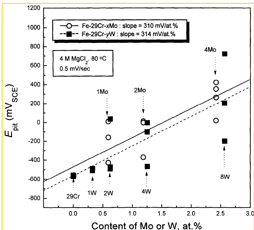
Fig. 4. Dependence of E_{pit} on atomic per cent of molybdenum or tungsten for Fe-29Cr ferritic stainless steels in 4 M MgCl_2 solution at 80°C
