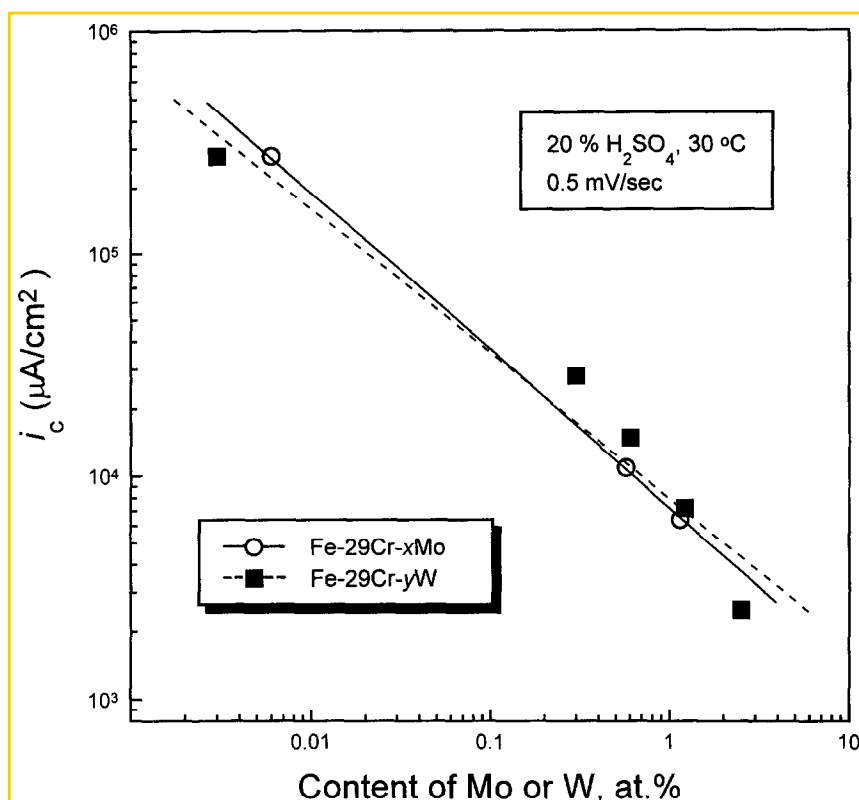
Fig. 12. i_c as a function of molybdenum or tungsten content for Fe-29Cr ferritic stainless steels in 20% \text{H}_2\text{SO}_4 solution at 30 °C
