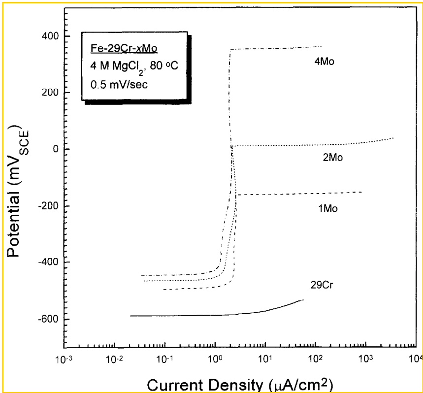
Fig. 1. Anodic polarization curves for Fe-29Cr ferritic stainless steels containing 0 to 4 wt% of molybdenum in 4 M MgCl 2 solution at 80 °C
